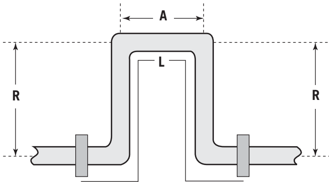
Figure 4 - Typical Expansion Loop
